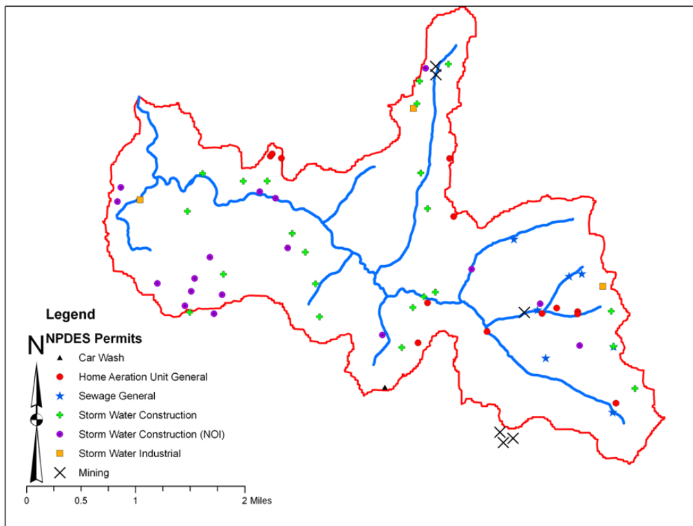
Figure 27: Locations and types of NPDES permits that discharge to West Run.
