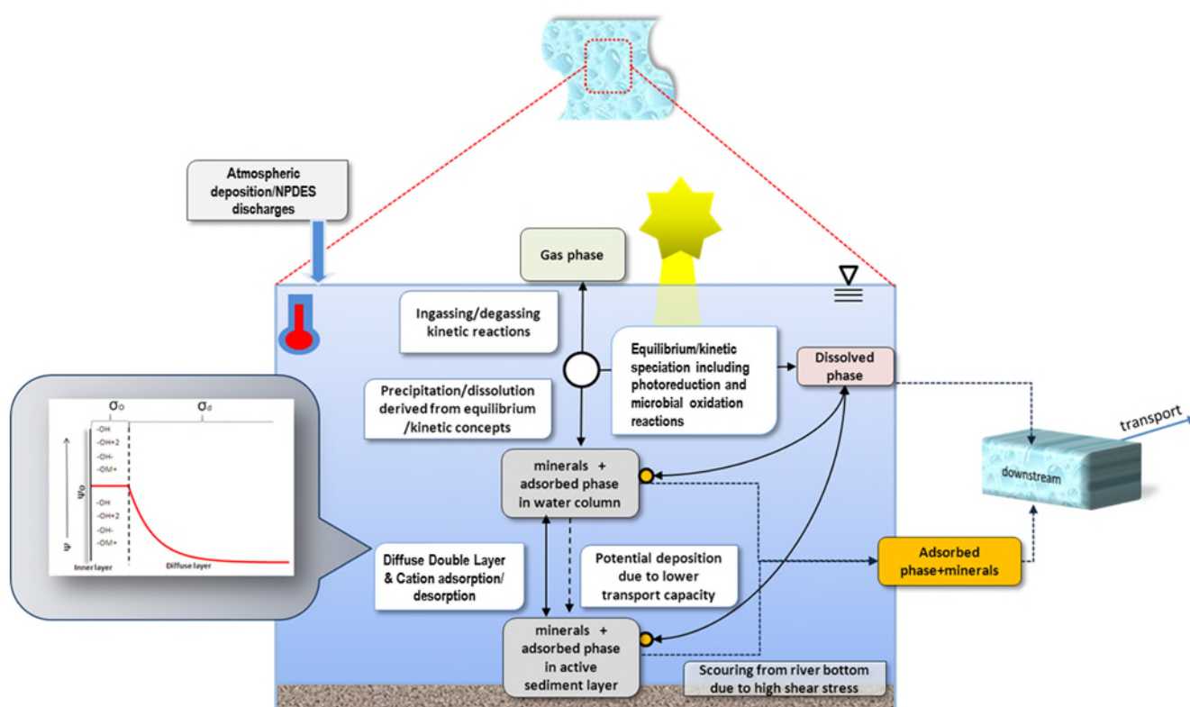
Figure 5-2. Stream components in MDAS
