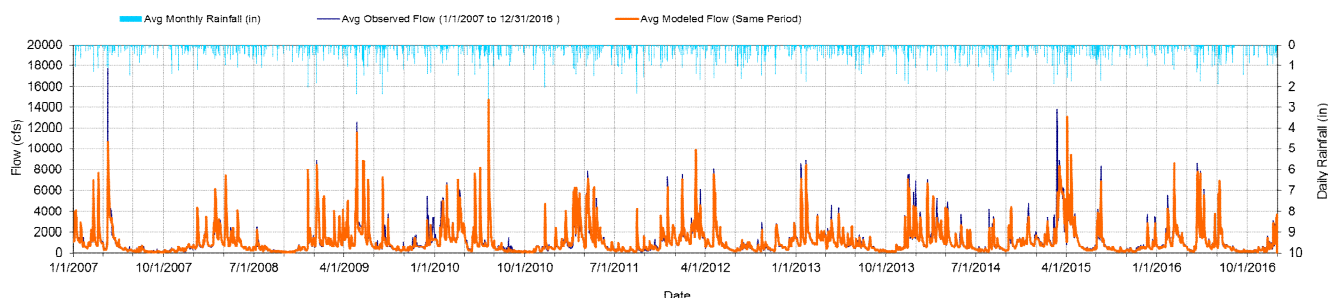
Figure 6-1. Comparison of simulated and observed flow from January 2007 to December 2016 for Upper Guyandotte River (WV-OGU)
