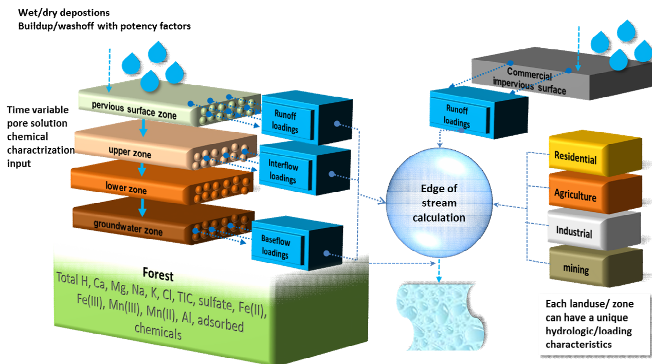
Figure 5-1. Land components of the LSPC-MDAS model
