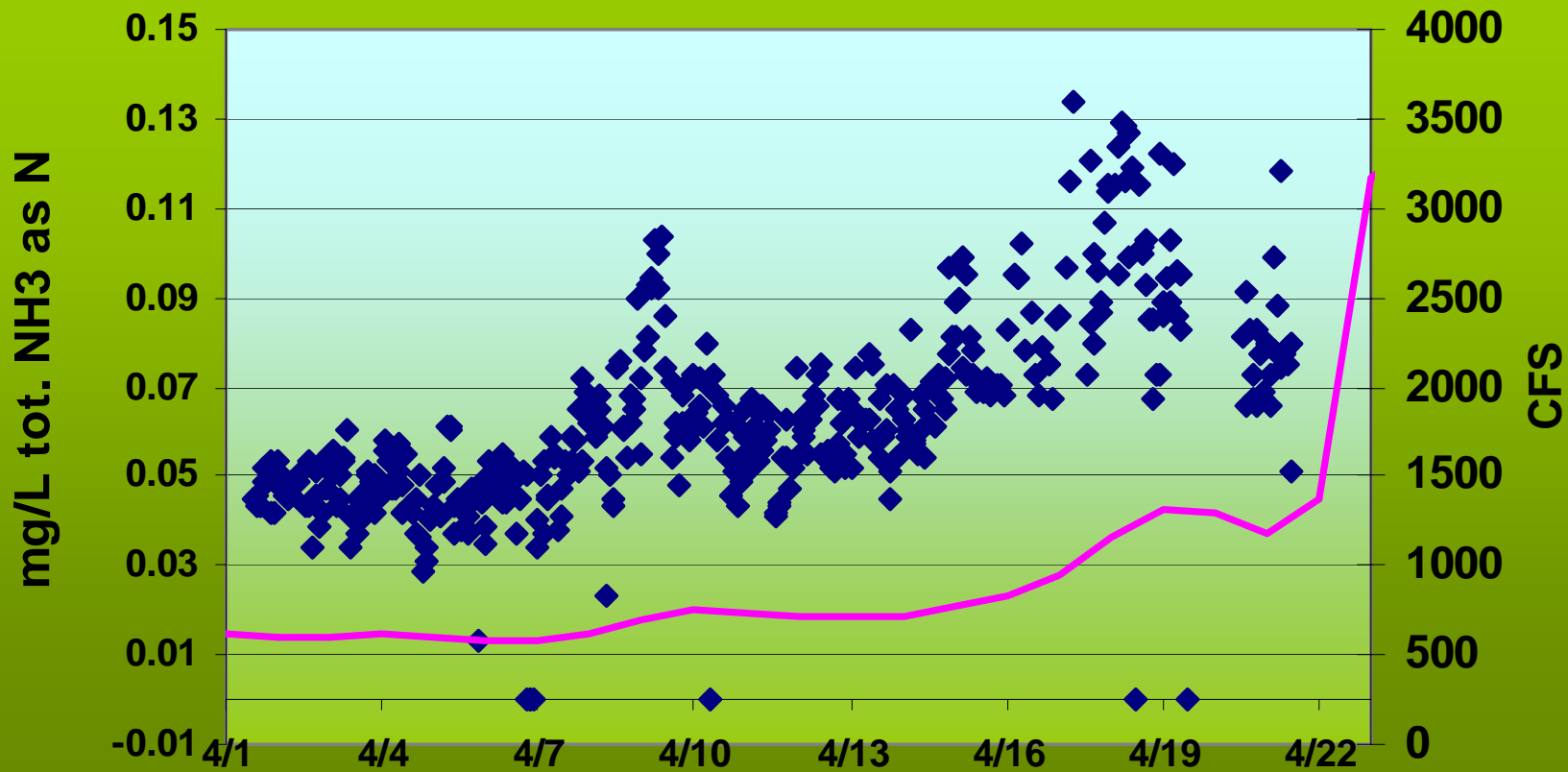
Hourly tot. NH3 at Luray
