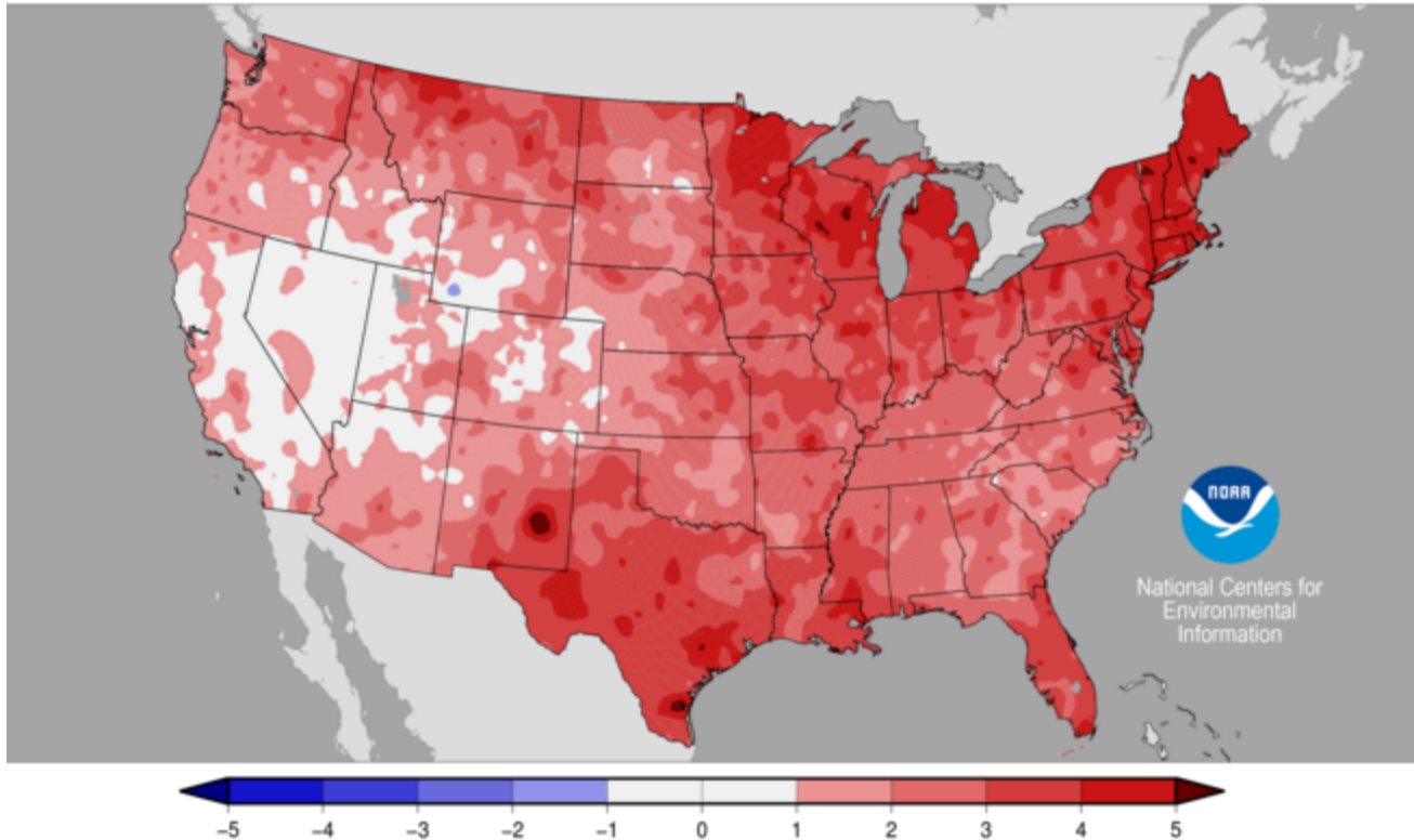
Figure 4. Mean temperature departures from average (from National Centers for Environmental Information National Oceanic and Atmospheric Administration ).
